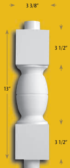
BAL 2229-13 • 6 5/8" Max. Repeat
