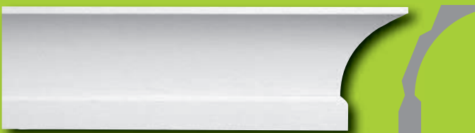
MD 1582RS • 6" Projection • 10" Height • 8'1/32" Length • ROUGH SAWN
