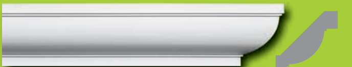
MD 1890 • 6 1/2" Projection • 7" Height • 12'0" Length
