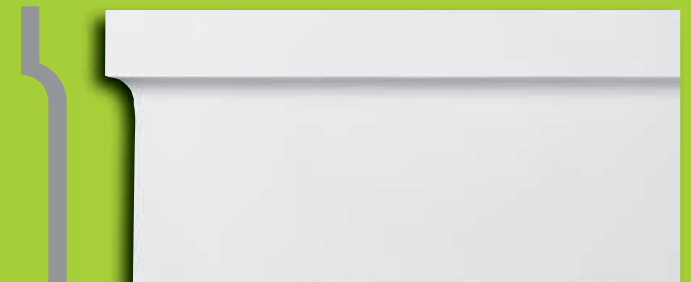
MD 1569 • 2 1/2" Projection • 15 1/4" Height • 12'0" Length
