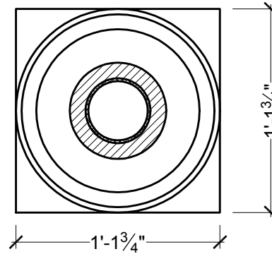
A SECTION
