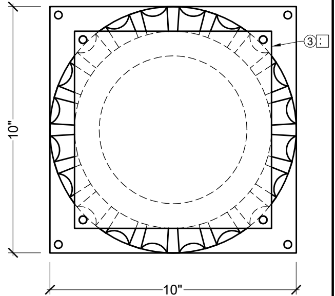
TOP VIEW SCALE: 1/4" = 1"
