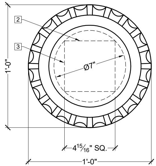
TOP VIEW SCALE: 3/16" = 1"
