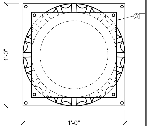
TOP VIEW SCALE: 3/16" = 1"
