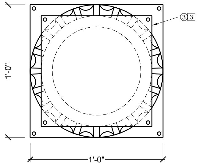
TOP VIEW SCALE: 3/16" = 1"
