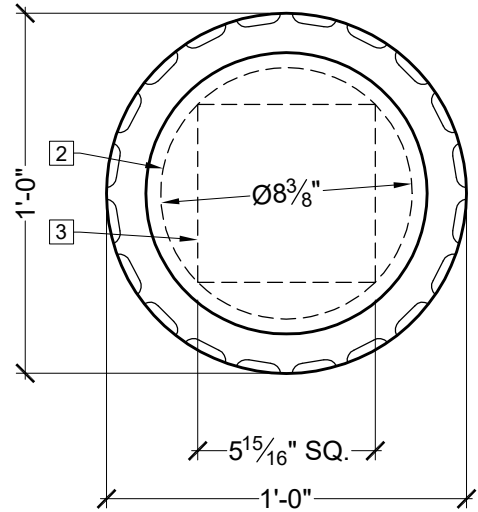
TOP VIEW SCALE: 5/32" = 1"
