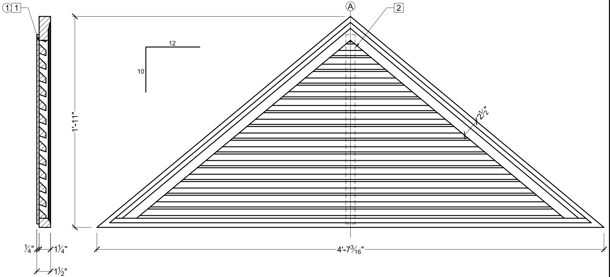
A SECTION VIEW
