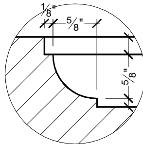
A RECESS DETAIL SCALE: 3/4" = 1"
