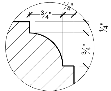
B CORNER DETAIL SCALE: 3/4" = 1"
