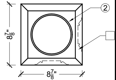
TOP VIEW OF CORNER POST
